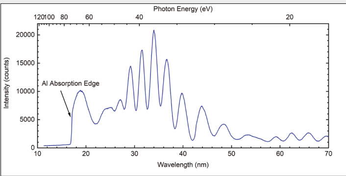
Figure 2. Left: Screenshot of our user-friendly software displaying the measurement of high-harmonic generated radiation in the XUV photon range. Right: Corresponding calibrated spectrum in wavelength and energy.
