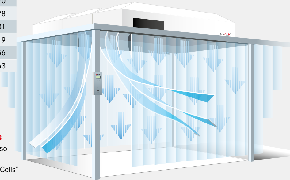
Partial view: A filter change can also be made from the clean room side.
