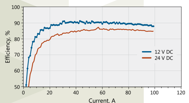
uniLDD efficiency.
