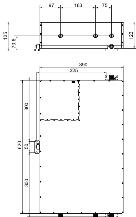
Dimensional drawing of Q-TUNE-HR (in mm)
