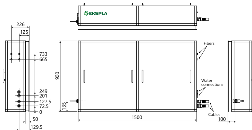
Fig 7. Typical APL601k laser system external dimensions
