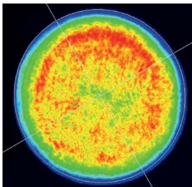
Fig 4. Typical High repetition rate APL amplifier system near field beam profile at 532 nm (imaged from SH crystal)
