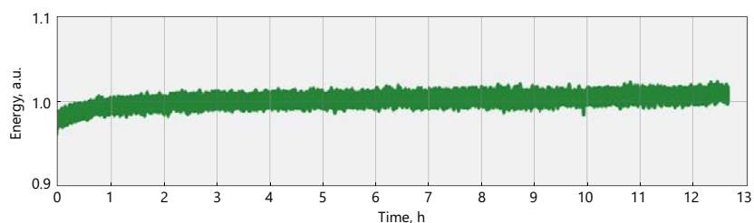
Fig 6. Typical long-term energy stability of High repetition rate APL amplifier system
