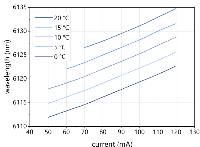
Typical mode hop free tuning of a nanoplus DFB ICL at 6125 nm by current and temperature
