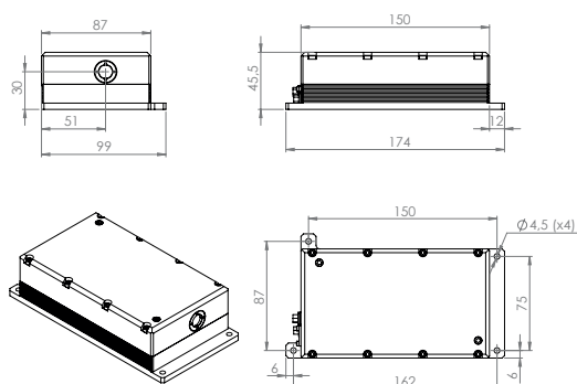
MPL2210 series laser head dimensions OEM version (in mm)
