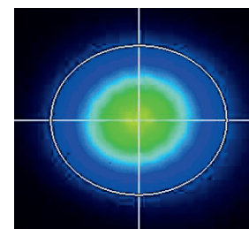
Typical beam intensity profile (20 cm from laser output) of MNL1342 series lasers
