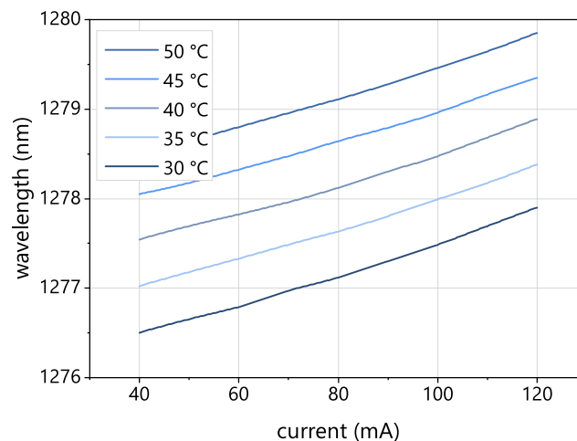
Typical mode hop free tuning of a nanoplus DFB laser at 1278 nm by current and temperature
